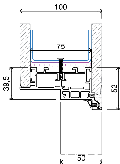
standard dimensions
