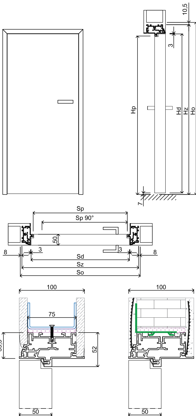
standard dimensions
