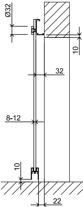
Version with rotulas
