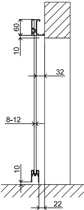
Version with cover strip
