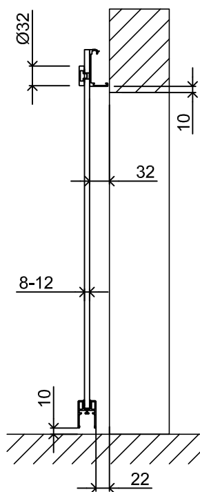
Version with rotulas
