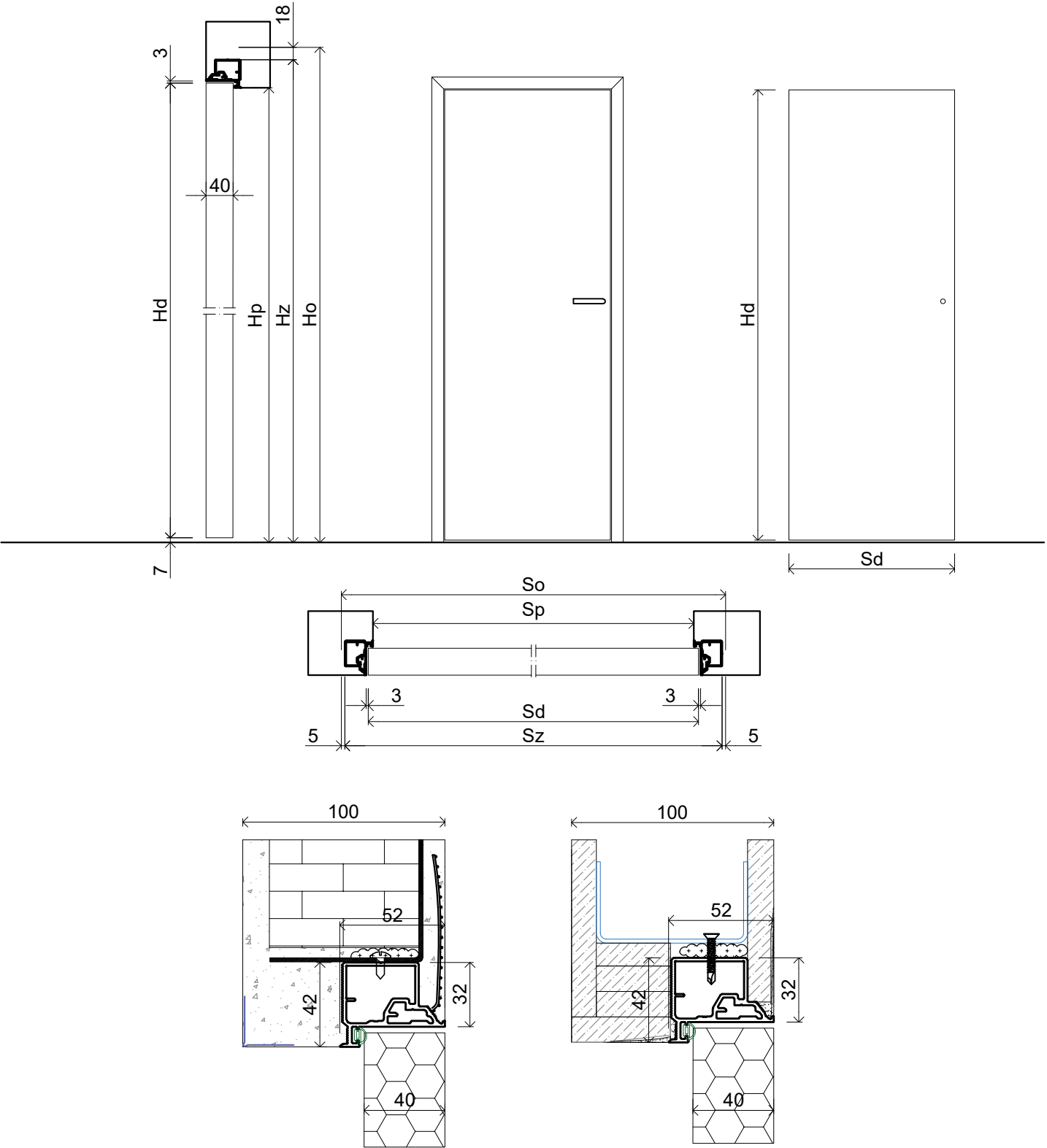
sample dimension
