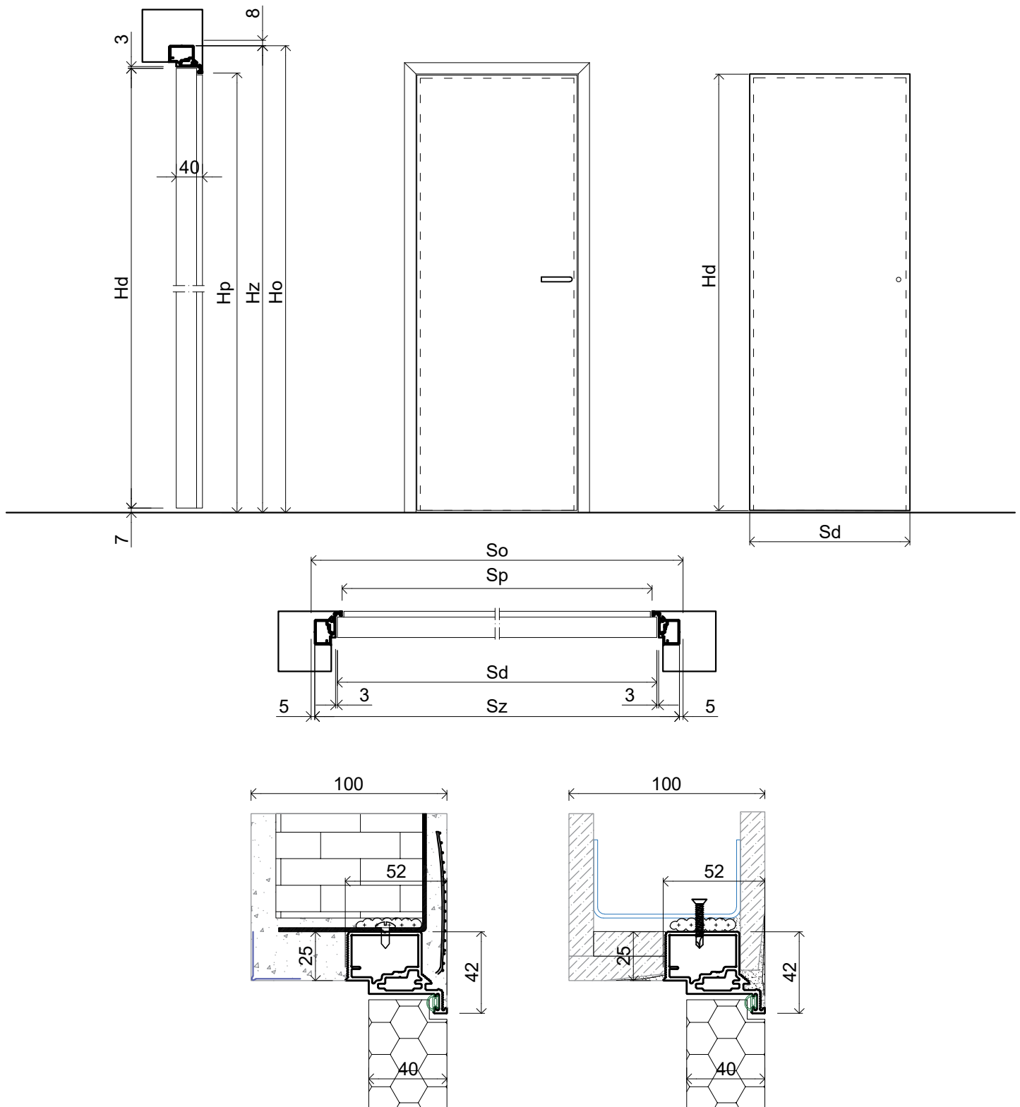
sample dimensions
