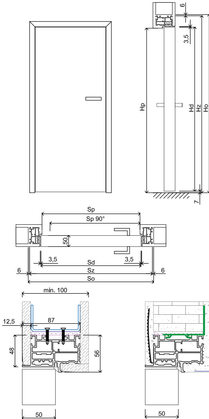
standard dimensions
