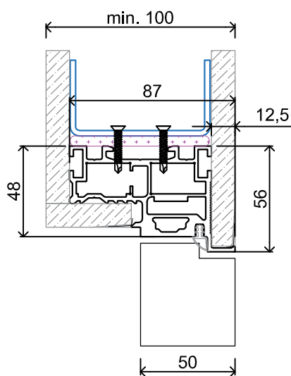
standard dimensions
